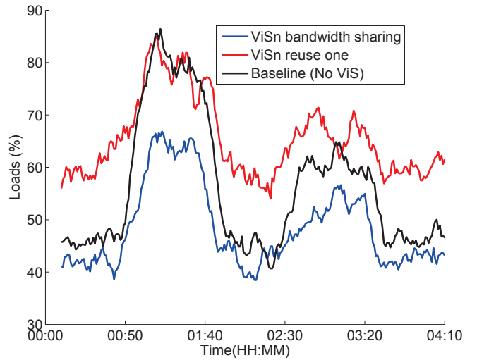
Fig. 8. Maximum loads evolution over time
