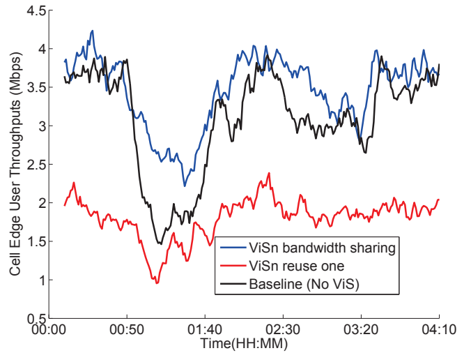
Fig. 7. Cell edge user throughputs evolution over time
