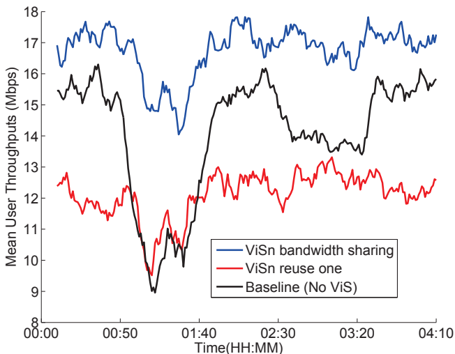
Fig. 6. Mean user throughputs evolution over time
